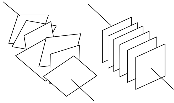
Fig. 3: SEM picture of isolated microcrystal on a Formvar-covered TEM grid. Notice the multilayered structure and sharpened extremities. Sketch of two (001)T type texture, with or without rotation.
